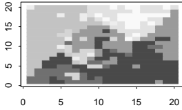
For 10 Groups, the indexes are: Jaccard = 0.356 Rand = 0.741
