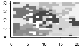
For 17 Groups, the indexes are: Jaccard = 0.203 Rand = 0.695
