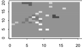
For 16 Groups, the indexes are: Jaccard = 0.37 Rand = 0.446
