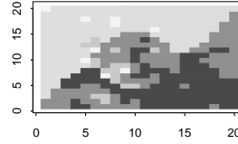
For 6 Groups, the indexes are: Jaccard = 0.414 Rand = 0.754
