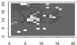
For 25 Groups, the indexes are: Jaccard = 0.362 Rand = 0.573
