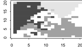
For 5 Groups, the indexes are: Jaccard = 0.406 Rand = 0.741
