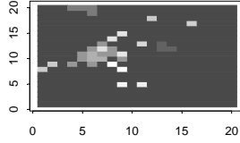
For 15 Groups, the indexes are: Jaccard = 0.371 Rand = 0.445
