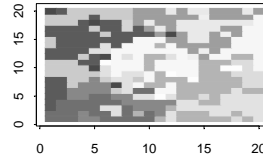
For 18 Groups, the indexes are: Jaccard = 0.207 Rand = 0.701
