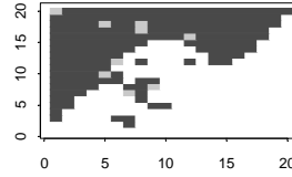
For 3 Groups, the indexes are: Jaccard = 0.658 Rand = 0.824
