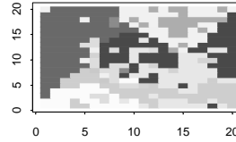
For 12 Groups, the indexes are: Jaccard = 0.29 Rand = 0.721
