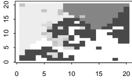
For 7 Groups, the indexes are: Jaccard = 0.409 Rand = 0.752
