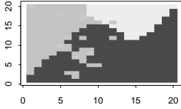
For 4 Groups, the indexes are: Jaccard = 0.523 Rand = 0.761
