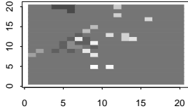
For 17 Groups, the indexes are: Jaccard = 0.37 Rand = 0.446
