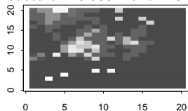
For 27 Groups, the indexes are: Jaccard = 0.358 Rand = 0.572
