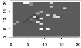
For 18 Groups, the indexes are: Jaccard = 0.37 Rand = 0.446
