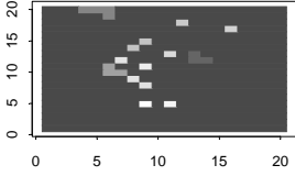
For 13 Groups, the indexes are: Jaccard = 0.372 Rand = 0.42
