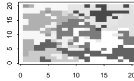
For 15 Groups, the indexes are: Jaccard = 0.227 Rand = 0.704
