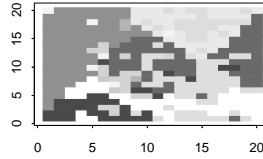
For 11 Groups, the indexes are: Jaccard = 0.292 Rand = 0.721
