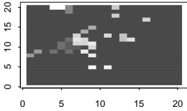
For 19 Groups, the indexes are: Jaccard = 0.37 Rand = 0.446
