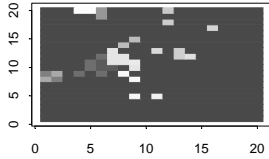
For 20 Groups, the indexes are: Jaccard = 0.368 Rand = 0.447
