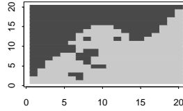
For 2 Groups, the indexes are: Jaccard = 0.679 Rand = 0.833
