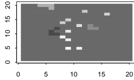
For 12 Groups, the indexes are: Jaccard = 0.372 Rand = 0.42
