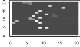
For 14 Groups, the indexes are: Jaccard = 0.37 Rand = 0.422
