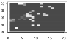
For 22 Groups, the indexes are: Jaccard = 0.366 Rand = 0.449
