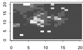
For 24 Groups, the indexes are: Jaccard = 0.364 Rand = 0.574
