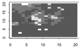
For 23 Groups, the indexes are: Jaccard = 0.365 Rand = 0.574
