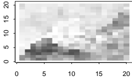
Original Data Set \alpha = 0.75
