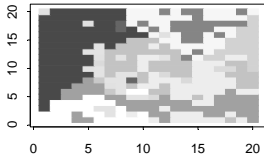
For 13 Groups, the indexes are: Jaccard = 0.29 Rand = 0.728
