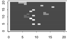
For 11 Groups, the indexes are: Jaccard = 0.371 Rand = 0.417
