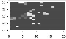
For 21 Groups, the indexes are: Jaccard = 0.367 Rand = 0.448
