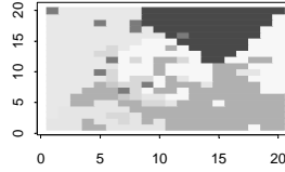
For 8 Groups, the indexes are: Jaccard = 0.389 Rand = 0.754
