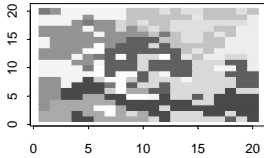
For 16 Groups, the indexes are: Jaccard = 0.224 Rand = 0.703
