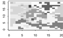
For 14 Groups, the indexes are: Jaccard = 0.227 Rand = 0.704
