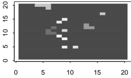
For 10 Groups, the indexes are: Jaccard = 0.372 Rand = 0.416
