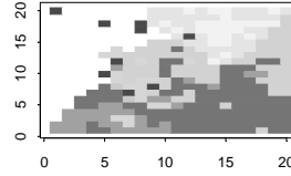
For 9 Groups, the indexes are: Jaccard = 0.357 Rand = 0.741
