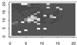
For 26 Groups, the indexes are: Jaccard = 0.362 Rand = 0.573
